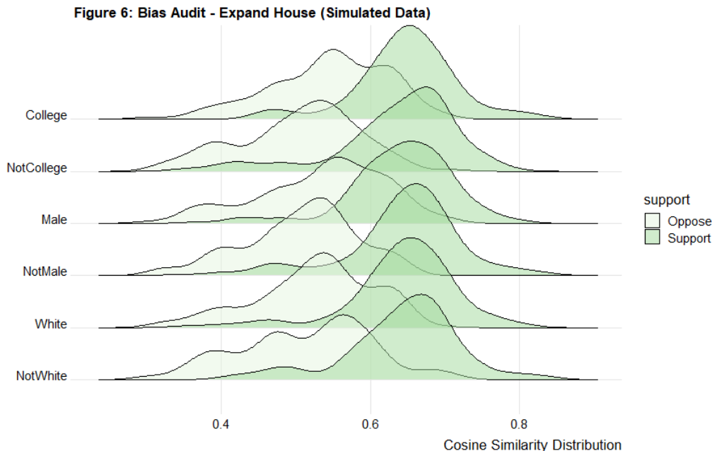
Figure 6: Distribution of simulated individual cosine similarity scores, conditional on demographics and position. N=600 design. Topic: Expansion of the U.S. House of Representatives
