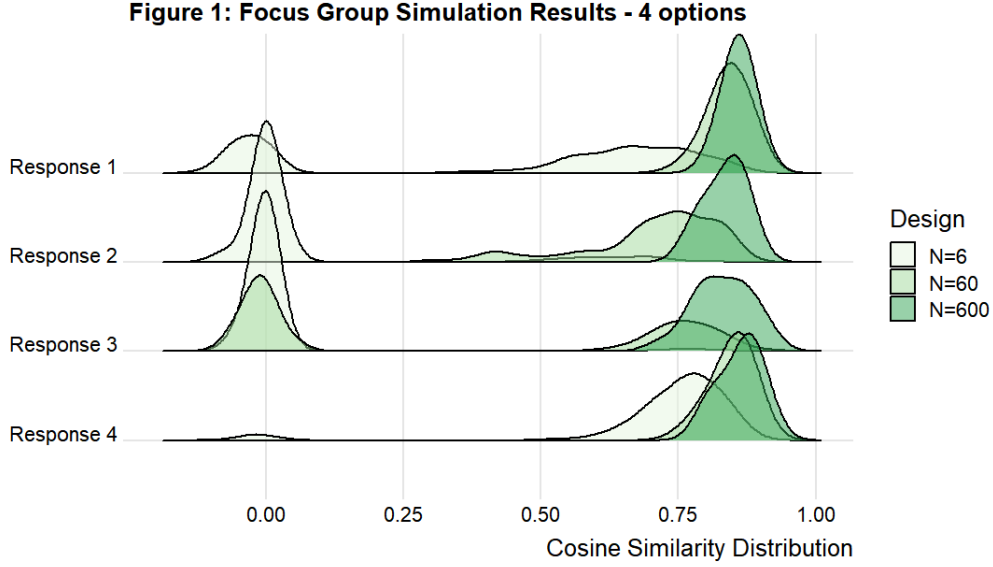
Figure 1: Distribution of pairwise cosine similarity scores, comparing between the small-N focus group design and the large-N design. Simulated focus group results on the topic of expanding nuclear power. Response 1: Implement rapid expansion and investment of nuclear power. Response 2: Maintain the current nuclear energy operations without change. Response 3: Phase out existing nuclear plants and halt new construction. Response 4: Prioritize researching improved implementations of nuclear power.
