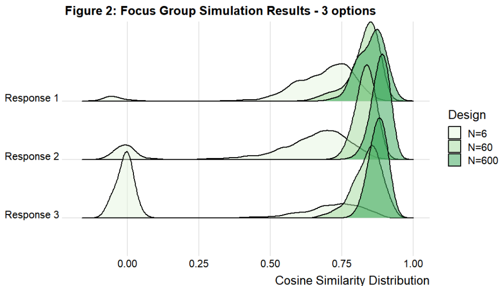
Figure 2: Distribution of pairwise cosine similarity scores, comparing between the small-N focus group design and the large-N design – three response options. Simulated focus group results on the topic of expanding nuclear power. Response 1: Implement rapid expansion and investment of nuclear power. Response 2: Maintain the current nuclear energy operations without change. Response 3: Phase out existing nuclear plants and halt new construction.
