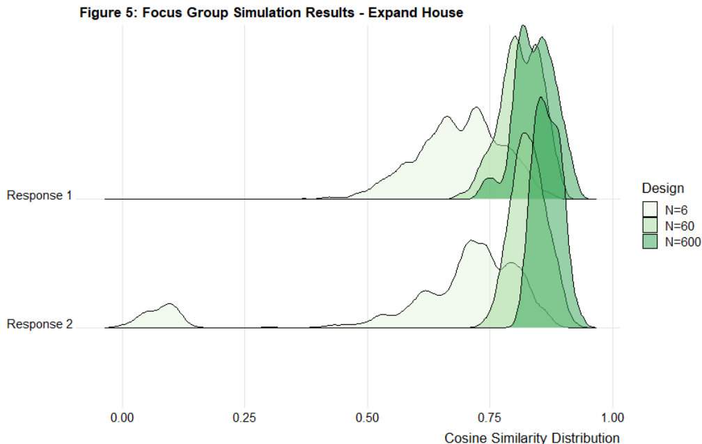
Figure 5: Distribution of pairwise cosine similarity scores, comparing between the small-N focus group design and the large-N design – two response options. Simulated focus group results on the topic of expanding the size of the U.S. House of Representatives. Response 1: In favor of expansion. Response 2: Opposed to expansion.
