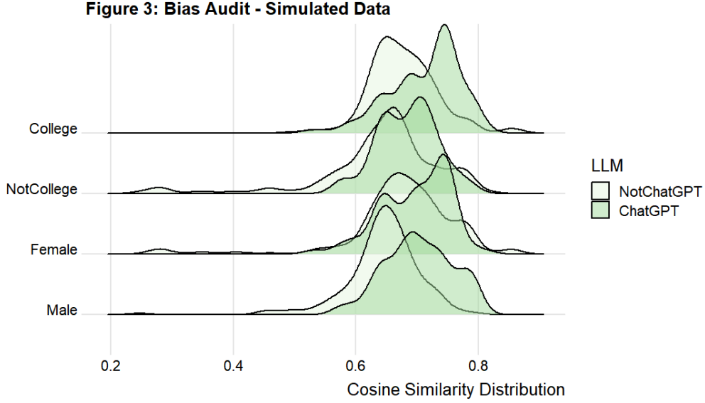
Figure 3: Distribution of simulated individual cosine similarity scores, conditional on demographics.
